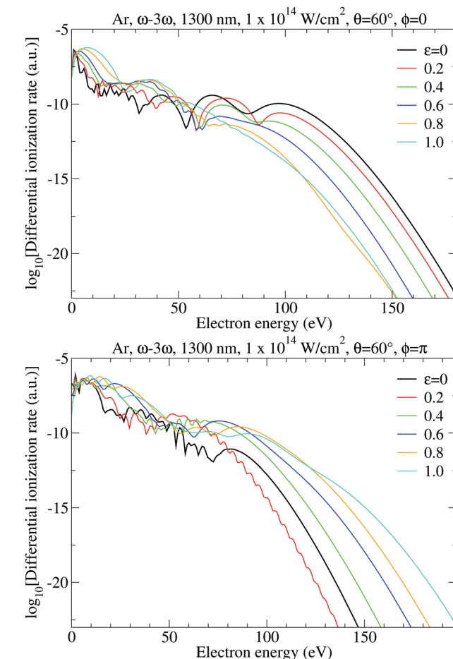
Fig. 10 The logarithm of the differential ionization rate of Ar atoms as a function of the photoelectron energy in electron volts for ionization by an \omega - 3\omega BEOTC field with the ellipticities \varepsilon = \varepsilon_1 = \varepsilon_2 as indicated. Both the direct and the rescattered electrons are included. The intensities of the field components are I_1 = I_2 = 1 \times 10^{14} \text{ W cm}^{-2} , the fundamental wavelength is 1300 nm, and the emission is in the direction \theta = 60^\circ . The relative phase is \phi = 0 (upper panel) and \phi = \pi (lower panel).
