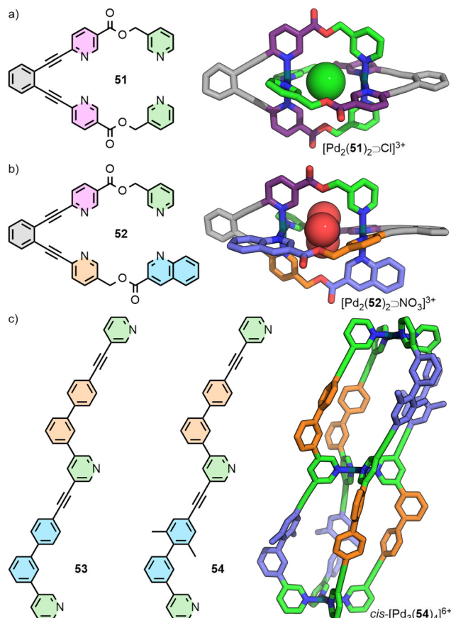
Fig. 10 Covalent trans -tethering of (a) identical ditopic ligand fragments enables access to \text{Pd}_2\text{L}_2 cages with a pseudo- \text{trans-Pd}_2\text{L}_4 cavity (SCXRD structure), and (b) different ditopic units generates a pseudo- \text{Pd}_2\text{L}_2\text{L}'_2 cavity of C_2 symmetry (SCXRD structure). (c) Unsymmetrical tritopic ligands 53 and 54 assemble to give trinuclear \text{cis-Pd}_3\text{L}_4 cages (PM6 model) where each cavity can be described as a pseudo- \text{Pd}_2\text{L}_2\text{L}'_2 environment.
