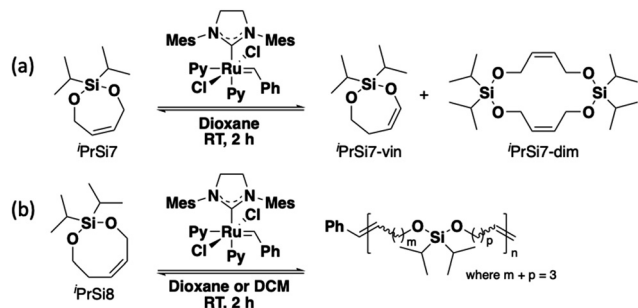
Scheme 1 Attempts at homopolymerization of bifunctional silyl ether monomers via ROMP. (A) Seven-membered i\text{PrSi7} forms isomerized cyclic vinyl silyl ether and cyclic dimer. (B) Eight-membered i\text{PrSi8} forms high molecular weight polysilylethers.
