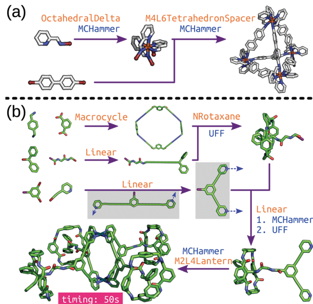
Fig. 5 Hierarchical construction (a) of a \Delta\text{-M}_4\text{L}_6 cage from an octahedral complex (this code was taken directly from the stk documentation) and (b) of a metallo-[5]rotaxane from ref. 100. Each purple arrow is a construction process, orange text is the topology graph used and blue text is the optimisation process used. The grey boxes show the (left) initial structure generated by stk , which must undergo conformer sampling to find the (right) conformer used for cage construction. MCHammer is a low-cost geometry optimisation function implemented in stk ; further optimisation would be required.
