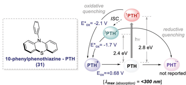
Scheme 17 Photophysical properties and redox potentials (vs. SCE in MeCN) of PTH (ref. 25c).
