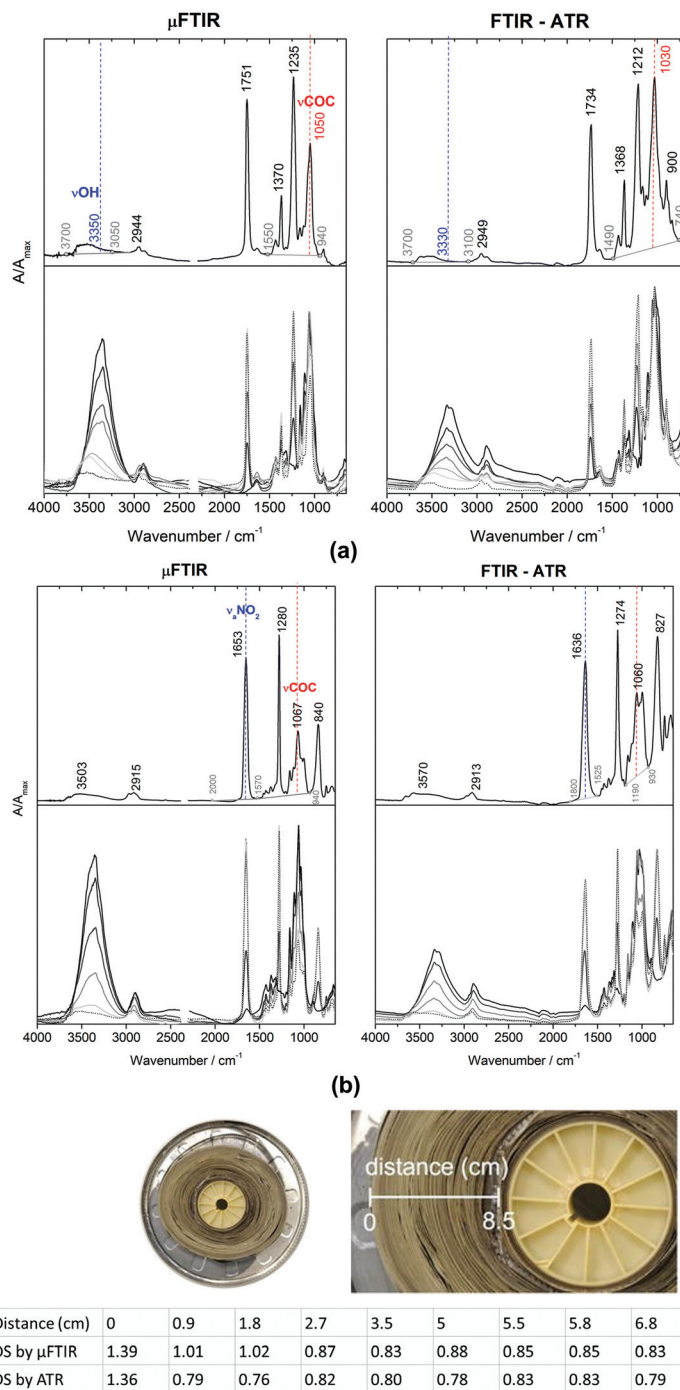
Fig. 9 Micro FTIR ( \mu -FTIR) in transmission mode and ATR-FTIR spectra of (a) CA and (b) CN, where 3330, 1030 \text{cm}^{-1} and 1636, 1060 \text{cm}^{-1} are used to produce DS values. (c) DS values of CA of a historical reef from the inner parts to outer parts acquired using \mu -FTIR and ATR-FTIR. Reproduced with permission, 155 copyright (2020) Springer Nature.
