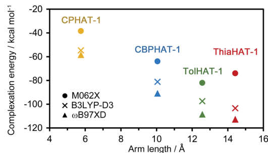
Fig. 8 Complexation energy–linker length plot of CPHAT-1 , CBPHAT-1 , TolHAT-1 , and ThiaHAT-1 , calculated at the B3LYP-D3/6-311G(d,p), M062X/6-311G(d,p) and \omega\text{B97XD}/6-311(\text{d},\text{p}) levels with the counterpoise method for BSSE correction.
