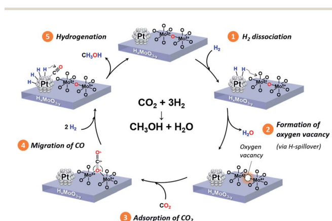
Scheme 2 Proposed reaction mechanism of CO 2 hydrogenation to produce methanol over the Pt/H x MoO 3−y catalyst.
