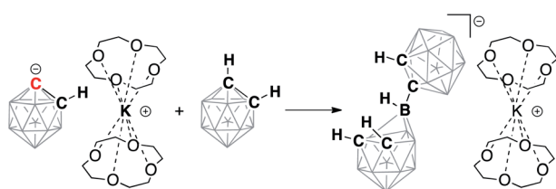
Scheme 4 Reaction of the strongly nucleophilic deprotonated free carboranyl anion with the parent protonated carborane cluster and the formation of the two-cage anion [\text{C}_4\text{B}_{20}\text{H}_{23}]^- . Unlabeled cluster vertices represent BH units.
