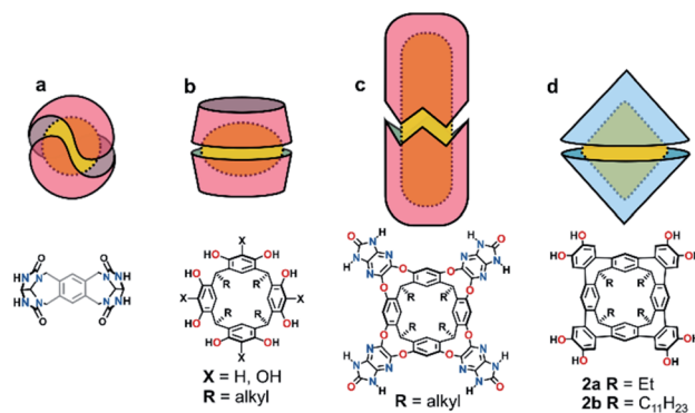
Fig. 1 Cartoon representations of hydrogen-bonded homo-dimeric capsules and chemical diagrams of their monomer units; (a) Rebek's tennis and softballs, (b) resorcin[4]arene dimers, (c) Rebek and de Medoza's cylindrical capsules and (d) the biconical capsules presented in this work.
