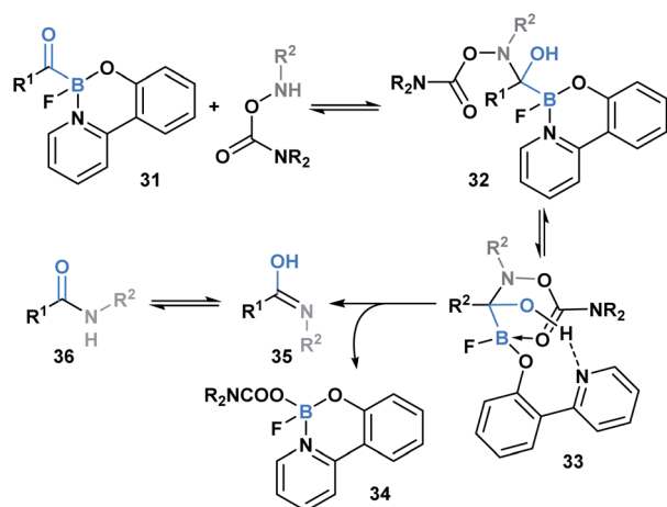
Scheme 9 Ligation between O-carbamoylhydroxylamines and monofluoroacylboronates proceeds via hemiaminal formation, pyridine dissociation/carboxyl association and elimination via a six-membered transition state.
