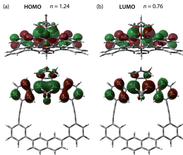
Fig. 1 (a) HOMO ( \psi_5 ) and (b) LUMO ( \psi_6 ) orbitals and their occupation numbers ( n ) calculated for S-DR3b at the CASSCF(2,2)/6-31G(d) level of theory.
