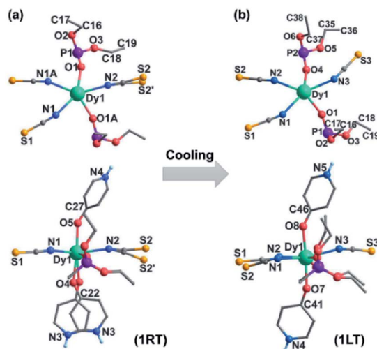
Fig. 3 Structural transformation from 1RT (a) into 1LT (b) upon cooling. The anthracene groups are omitted for clarity.
