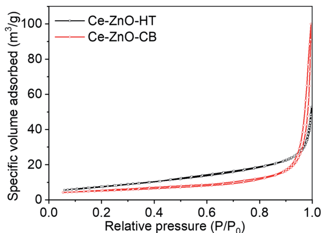
Fig. 4 Adsorption and desorption isotherm of Ce-ZnO-CB and Ce-ZnO-HT NPs.
