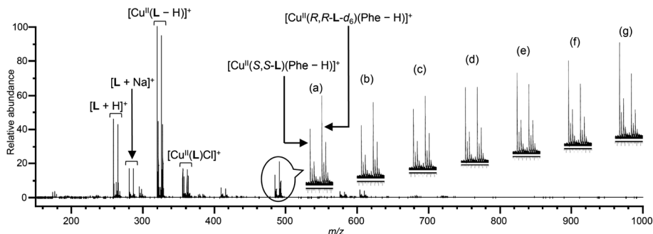
Fig. 3 Mass spectra of a mixture of Cu II /S,S-L/R,R-L- d 6 /Phe in the presence of K 2 CO 3 in water/methanol (1/100, v/v). [CuCl 2 ] 0 = 9.90 × 10 −5 M, [S,S-L] 0 = [R,R-L- d 6 ] 0 = 5.94 × 10 −5 M, and [Phe] 0 = [K 2 CO 3 ] 0 = 9.90 × 10 −6 M. [CuCl 2 ] 0 /[S,S-L] 0 /[R,R-L- d 6 ] 0 /[Phe] 0 = 1.0/0.6/0.6/0.1. Optical purity of Phe (a) S 100% ee, (b) S 70% ee, (c) S 30% ee, (d) 0% ee (racemic), (e) R 30% ee, (f) R 70% ee, and (g) R 100% ee.
