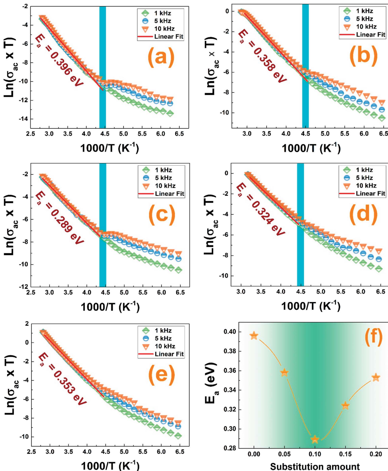
Fig. 11 (a–e) Variation of \ln(\sigma_{ac} \times T) vs. 1000/T for \text{La}_{1-2x}\text{Ba}_x\text{Bi}_x\text{FeO}_3 (x = 0.00, 0.05, 0.10, 0.15 and 0.20) compounds, respectively; (f) the variation of the activation energy as function of the substitution amount for grain and grain boundaries contributions.
