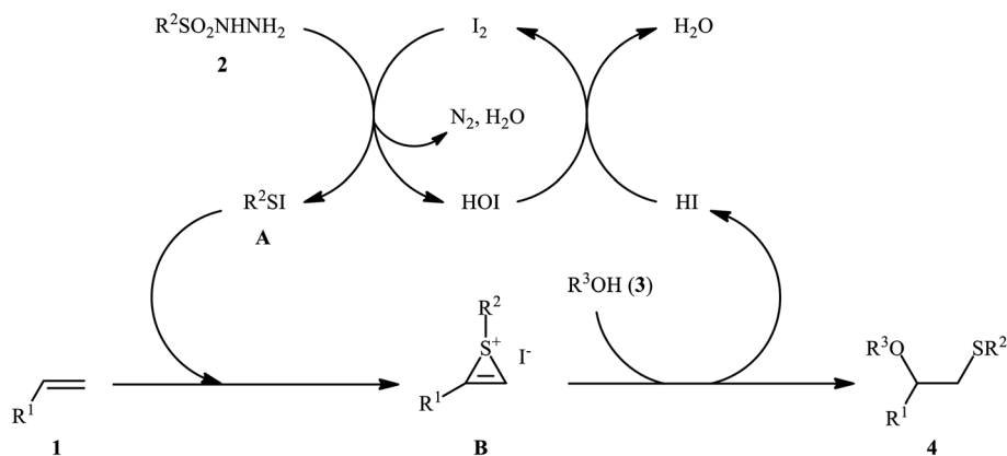
Scheme 2 I 2 -catalyzed alkoxy-sulfenylation of alkenes 1 with sulfonyl hydrazides 2 and alcohols 3 .
