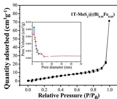
Fig. 6 Nitrogen gas adsorption-desorption isotherm distribution curve for 1\text{T-MoS}_2@(\text{Bi}_{0.40}\text{Fe}_{0.60})\text{VO}_4 at 77 K. Inset: pore volume vs. pore diameter curve from BJH method.
