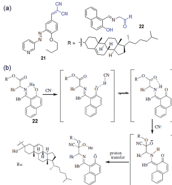
Fig. 17 (a) Structures of compounds 21 and 22 . (b) Probable mechanism of cyanide sensing by 22 . Reproduced with permission from ref. 210.
