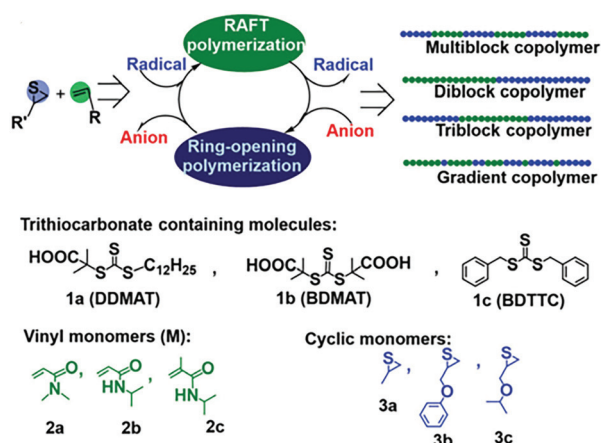
Fig. 4 Interconvertible hybrid copolymerizations of AROP and RAFT. Reproduced from ref. 23 with permission from the Royal Society of Chemistry, copyright 2019.
