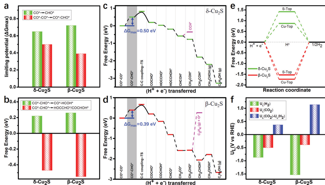
Fig. 3 Free energy of the hydrogenation step of (a) \text{CO}^* \rightarrow \text{CHO}^* and \text{CO}^* \rightarrow \text{CHO}^* \rightarrow \text{HOCCHO}^*/\text{COCHOH}^* . Free energy diagrams of \text{CO}^* \rightarrow \text{CHO}^* hydrogenation to \text{C}_2\text{H}_5\text{OH} on (c) \delta -Cu 2 S and (d) \beta -Cu 2 S. Limiting potential is obtained from the maximum free energy change ( \Delta G_{\text{max}} ) of the whole reaction process, which is marked by blue lines. (e) Free energy profiles of the HER on \delta -Cu 2 S (green line) and \beta -Cu 2 S (red line). (f) Limiting potentials for the CO 2 RR U_L(\text{CO}_2) , HER U_L(\text{H}_2) and difference U_L(\text{CO}_2) - U_L(\text{H}_2) on \delta -Cu 2 S and \beta -Cu 2 S monolayers.
