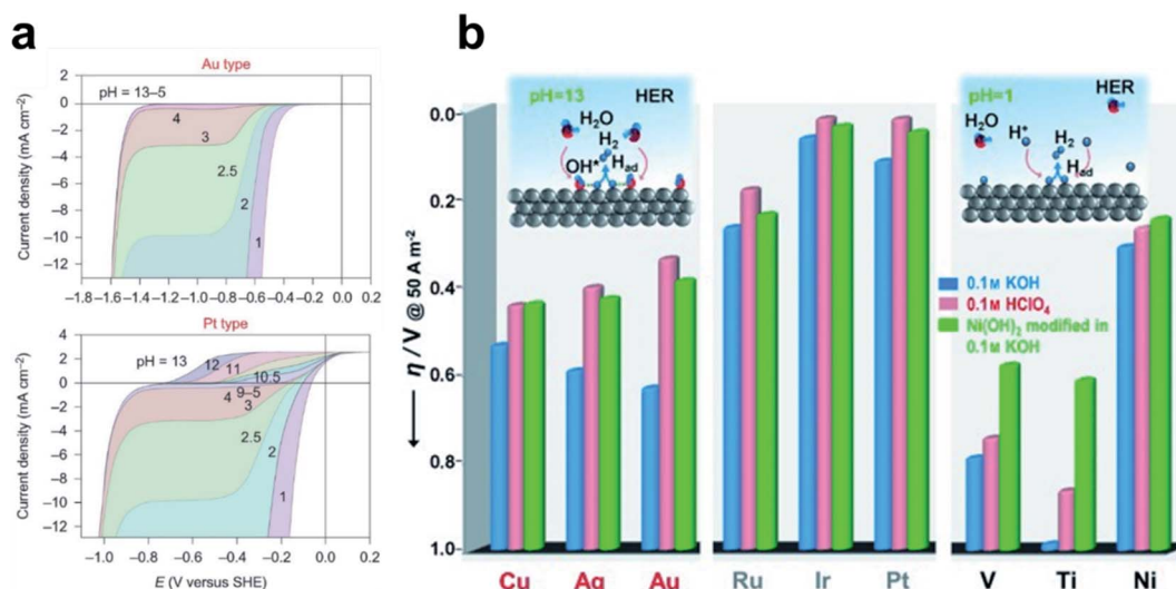
Fig. 1 (a) pH-dependent current–potential polarization curves at rotation rates of 1600 rpm and sweep rate of 50 \text{ mV s}^{-1} for Au(111) and Pt(111). Reproduced from ref. 93 Copyright 2013, Springer Nature. (b) Overpotential \eta required for a 5 \text{ mA cm}^{-2} current density, in 0.1 \text{ M HClO}_4 and 0.1 \text{ M KOH} for bare metal surfaces (Cu, Ag, Au, Ru, Ir, Pt, V, Ti and Ni) and \text{Ni}(\text{OH})_2 -modified surfaces. Reproduced from ref. 46. Copyright 2012, Wiley.
