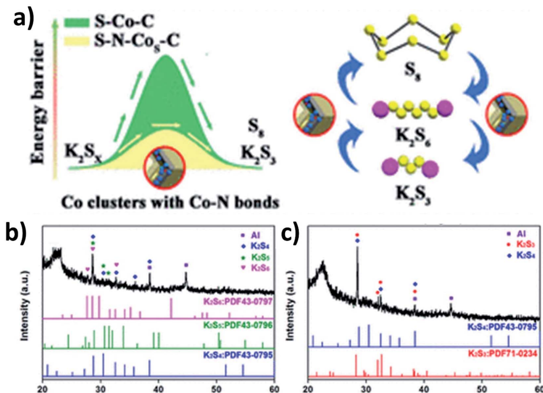
Fig. 16 (a) Schematic illustration of the catalytic mechanism of N-Co for the polysulphide conversion reaction, and XRD analysis of S-N-Co/C discharged to (b) 1 V and (c) 0.5 V. Reproduced with permission. Copyright 2020, American Chemical Society.
