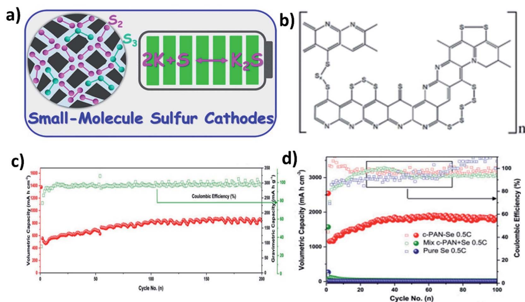
Fig. 15 (a) Schematic illustration of the conversion of small S_2 - S_3 molecules directly to K_2S . Reproduced with permission. Copyright 2019, American Chemical Society. (b) Schematic of the structure of SPAN. Reproduced with permission, Copyright 2020, Wiley-VCH. (c) Cycling performance of Se_1/PAN at a rate of 5C and (d) the comparison of the cycling performance of Se_1/PAN , physically mixed Se + PAN and pure Se. Reproduced with permission. Copyright 2017, Elsevier.
