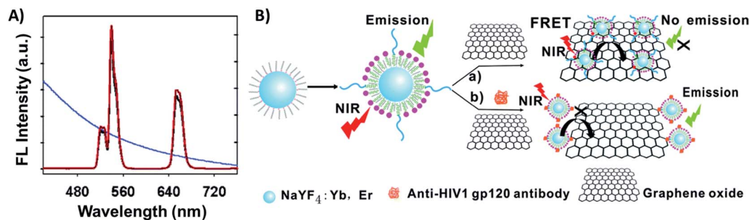
Fig. 21 UCNP-GO FRET sensor for HIV antibody detection. (A) UC fluorescence spectra of peptide-functionalized UCNP and the absorption spectrum of GO (blue curve). (B) Schematic illustration of the upconversion FRET-based biosensor for the detection of anti-HIV-1 gp120 antibodies. Modified with permission from ref. 202. Copyright 2014, The Royal Society of Chemistry.
