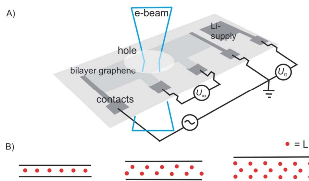
Fig. 1 Illustration of in situ transmission electron microscopy of the Li-intercalation process in suspended 2L graphene, triggered in a device. (A) Illustration of the device on a Si 3 N 4 -covered Si substrate. (B) from left to right: side-views of expected ‘conventional’ C 6 LiC 6 configuration and of the experiment matching structures with 2L Li crystal and 3L Li crystal. 15
