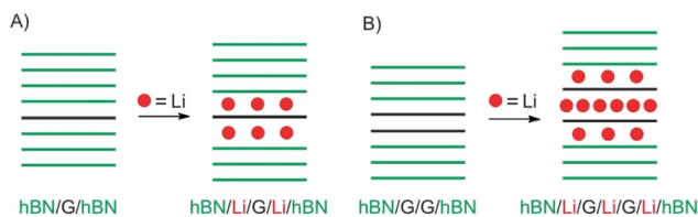
Fig. 5 Study of device-based electrochemical intercalation of Li in heterostructures of (A) graphene (G) artificially intercalated in hBN and (B) 2L graphene artificially intercalated in hBN.
