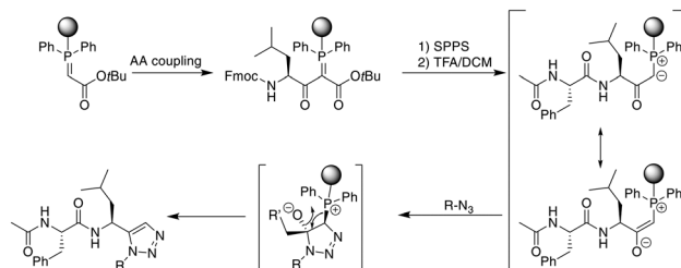
Scheme 37 Synthetic scheme for the metal-free synthesis of 1,5-substituted triazole peptides. AA = amino acid.
