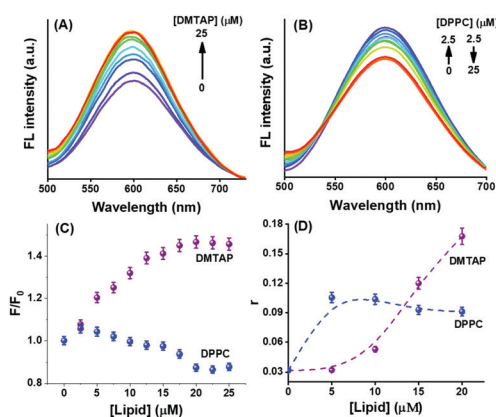
Fig. 3 Influence of the added GUVs from (A) DMTAP and (B) DPPC lipids on the fluorescence emission of the GSH-AuNCs in aqueous buffer under normal conditions ( \lambda_{\text{ex}} = 375 nm); (C) provides a comparative plot of the relative fluorescence yields due to the interactions and (D) shows the steady state fluorescence anisotropy ( r ) plots for the two cases (the dashed lines are to guide the view).
