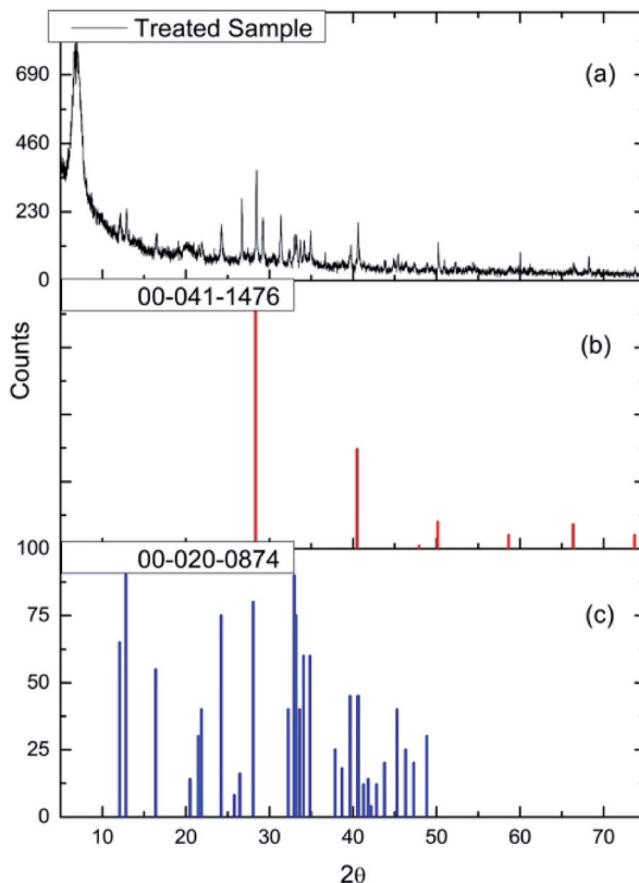
Fig. 15 (a) The X-ray diffraction pattern of the dichlorine pre-treated \text{CuCl}_2/\text{KCl}/\text{attapulgite} catalyst (chlorine exposure = 12.8 \text{ mmol Cl}_2 \text{ per g}_{(\text{cat})} ). Reference diffraction patterns for (b) KCl (red) and (c) \text{KCuCl}_3 (blue).
