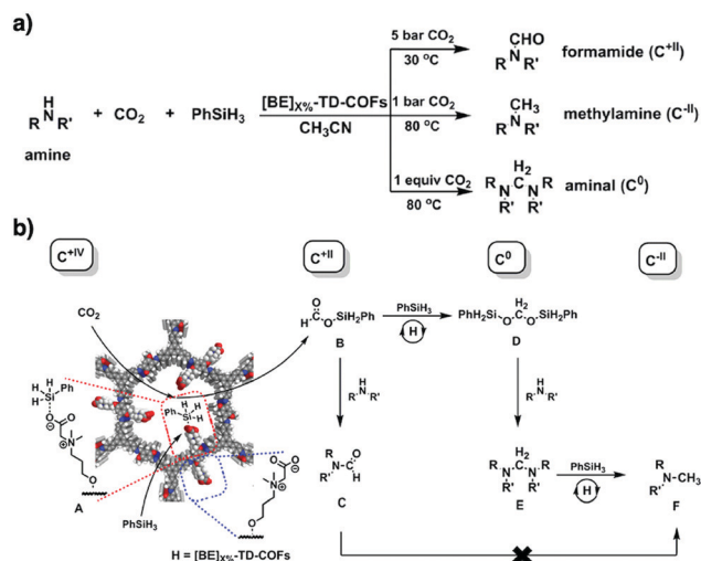
Fig. 112 (a) Using [BE]_{x\%} -TD-COFs as catalysts for hierarchical reduction of CO_2 with amines to afford formamides, aminals and methylamines. (b) Proposed reaction mechanism of hierarchical reduction of CO_2 catalysed by [BE]_{x\%} -TD-COFs (H) with amines and PhSiH_3 to gain formamides (C), aminals (E) and methylamines (F). Adapted with permission from ref. 229, Copyright 2018 ACS.
