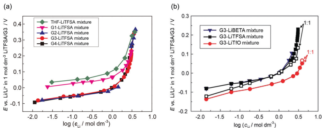
Fig. 3 Plots of the \text{Li/Li}^+ electrode potential against a common logarithm of the Li salt concentration in (a) G4 (tetraglyme), G3 (triglyme), G2 (diglyme), G1 (monoglyme), and THF-LiTFSA mixtures; (b) G3-LiTfO, -LiTFSA, and -LiBETA mixtures at 30 °C. Reference electrode was \text{Li/Li}^+ in 1 mol \text{dm}^{-3} LiTFSA/G3. (b) was reprinted with permission from ref. 59 Copyright 2015 PCCP Owner Societies.
