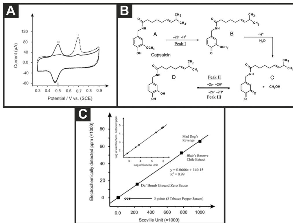
Fig. 2 (A) The first (dotted lines) and second (solid line) scans for the AdsSV of 100 μM capsaicin on the MWCNT-BPPGE in a 0.05 M Britton–Robinson buffer solution at pH 1.0, after 1 min accumulation in open circuit conditions; scan rate: 100 mV s -1 . (B) Proposed electrochemical mechanism for the electrochemical oxidation/reduction of capsaicin. (C) Measured value of capsaicin concentration in ppm (electrochemically detected ppm) versus the average Scoville units for six hot pepper sauces. Inset: log of the electrochemically detected ppm versus log of the average Scoville units for six hot pepper sauces. Scheme and images reproduced with permission from ref. 40. Copyright Royal Society of Chemistry 2008. 40
