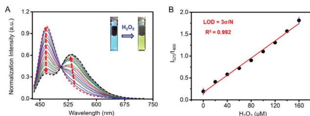
Fig. 2 Sensitivity and selectivity of Cm-Np-B@BSA (5/50 \mu M) for H 2 O 2 detection. (A) Fluorescence spectral response of Cm-Np-B@BSA (5/50 \mu M) to H 2 O 2 at the concentration of 0–200 \mu M; (B) linear detection range and limit of detection (LOD) of Cm-Np-B@BSA (5/50 \mu M). All measurements were carried out in PBS buffer, pH 7.4, excitation wavelength: 410 nm.
