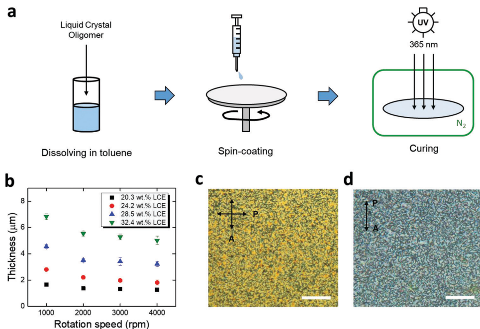
Fig. 3 (a) Schematic illustration of LCE spin-coating process. (b) Thickness of spin-coated LCE films as functions of LCE concentration and rotation speed (mean \pm SD, n = 3 ). Polarized optical micrographs of spin-coated LCE (c) on a gold trace (viewed in reflection mode) and (d) on a twisted nematic LCE substrate (viewed in transmission mode). (Scale bars = 30 μm.)
