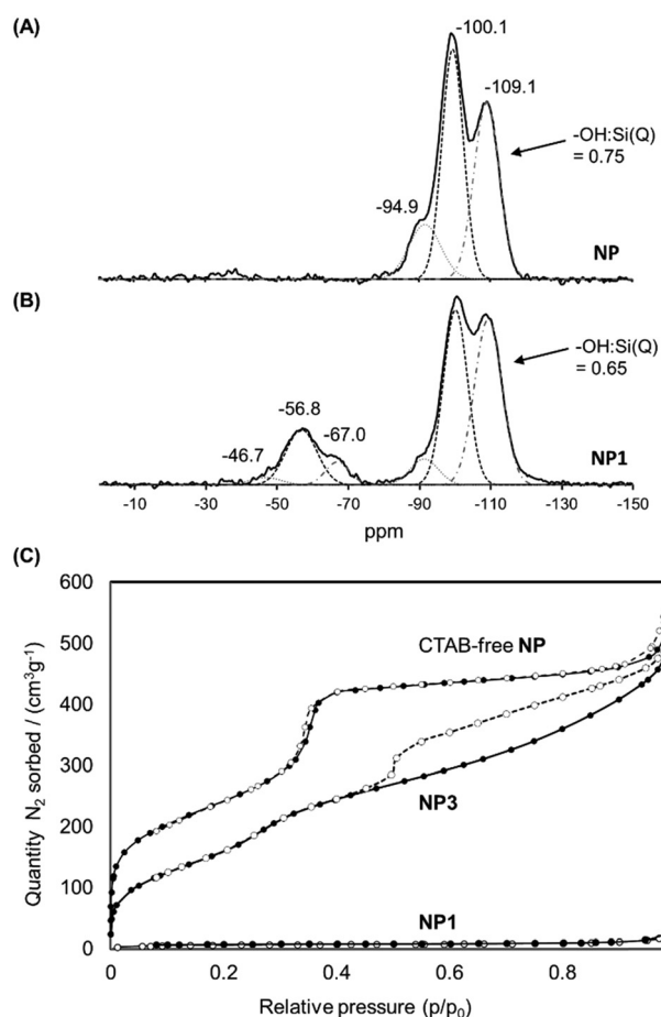
Fig. 5 Solid state 29 Si NMR spectra of NP (A) and NP1 (B). (C) Isotherms of CTAB-free NP , NP1 and NP3 obtained by nitrogen sorption analyses.
