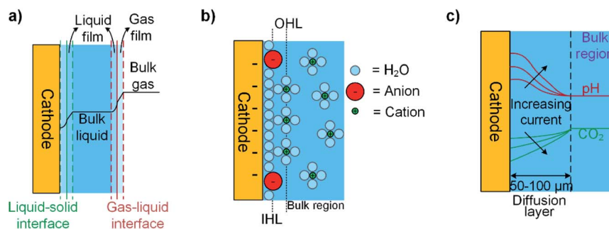
Fig. 4 Schematic illustrations of (a) the concentration profile of \text{CO}_2 across gas, liquid, and solid interfaces; (b) the electrochemical double layer with specifically adsorbed anions at the inner Helmholtz layer and solvated cations at outer Helmholtz layer; and (c) changes in \text{CO}_2 and pH next to the diffusion layer at increasing current density in a system where \text{CO}_2 is supplied from the bulk electrolyte.
