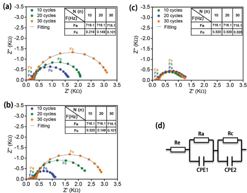
Fig. 4 EIS spectra of ASSEBs with (a) bare \text{LiCoO}_2 electrode, (b) LCO-coating protected \text{LiCoO}_2 electrode, and (c) LCO + CB-coating protected \text{LiCoO}_2 electrode after 10, 20, and 30 cycles of charge/discharge. The inset tables show the critical frequency values on top of the high frequency semi-circle ( F_a ) and low frequency semi-circle ( F_c ) at different cycles of charge/discharge, respectively. (d) The equivalent circuit for fitting the EIS spectra.
