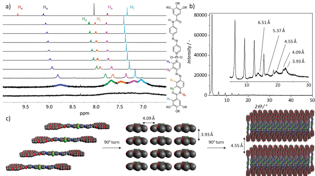
Fig. 4 (a) Solvent-dependent ^1\text{H} NMR spectra of C1 at 298 K ( c = 1 \times 10^{-3} M) from 100% \text{THF-d}_8 (top) to 10% \text{THF-d}_8 and 90% \text{D}_2\text{O} (bottom) in 10% steps with a scheme clarifying the colour code depicted on the side. (b) XRD-diffraction pattern ( \lambda = 1.5406 Å) of a thin film of the aggregate of C1 obtained from drop casting a 1 \times 10^{-3} M solution (THF : water 9 : 1) between 2 and 50^\circ with an inset of the region between 4.5 and 30^\circ . The sharp reflexes are allocated to originate from the d -spacing between Pt atoms. (c) Cartoon representation of the 3D packing model derived from combining the results of the ^1\text{H} NMR and XRD experiments with the most important intermolecular distances highlighted. The 2D layers depicted on the right are capable of stacking indefinitely during the sample preparation (drying), which enables analysis with XRD. Only two are shown for clarity.
