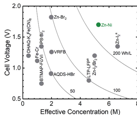
Fig. 1 Theoretical volume energy densities of some representative aqueous flow battery chemistries including VRFB, 11 Fe–Cr, 33 BTMAP-Fc/Vi, 16 Zn–Br 2 , 34 LTP–LFP 3,4 , Zn–I 2 /Br 2 , 35 Zn–I 2 , 38 PS–Br 2 (ref. 36) and DHAQ– \text{K}_4\text{Fe}(\text{CN})_6 , 14 and AQDS–HBr. 9 Abbreviations: BTMAP-Fc: 1,1'-bis[3-(trimethylammonio)propyl]ferrocene dichloride, BTMAP-Vi: bis[3-(trimethylammonio)propyl]viologen tetrachloride, PS: polysulfide, AQDS: 9,10-antraquinone-2,7-disulphonic acid, DHAQ: 2,6-dihydroxyanthraquinone, LTP: \text{LiTi}_2(\text{PO}_4)_3 , LFP: \text{LiFePO}_4 .
