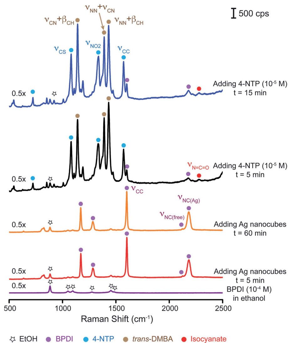
Fig. 5 Raman spectrum recorded from a BPDl solution ( 10^{-4} M) in ethanol and time-elapsd SERS spectra collected at different time points from an ethanolic suspension of Ag nanocubes and BPDl before and after the addition of 4-NTP solution in ethanol ( 10^{-5} M).
