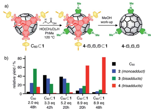
Fig. 4 (a) Cage-templated synthesis of N-methylfulleropyrrolidine trisadducts; (b) relative yields (based on HPLC integration) for unreacted C 60 (black) and Prato adducts 2 (mono, blue), 3 (bis, green) and 4 (tris, red) for control experiment and cage-templated reactions.
