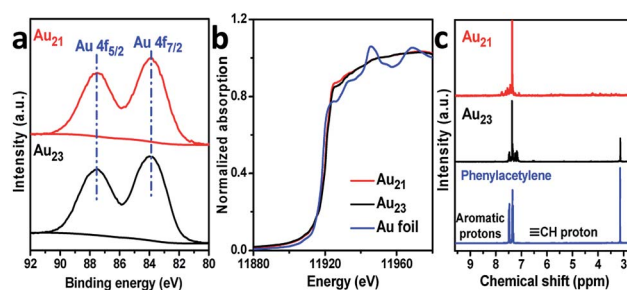
Fig. 5 (a) Au 4f XPS and (b) Au L 3 -edge XANES profiles of \text{Au}_{21}(\text{SR})_{12}(\text{Ph}_2\text{PCH}_2\text{PPh}_2)_2 and \text{Au}_{23}(\text{SR})_{16} . (c) The ^1\text{H} NMR spectra of Au-acetylide species.
