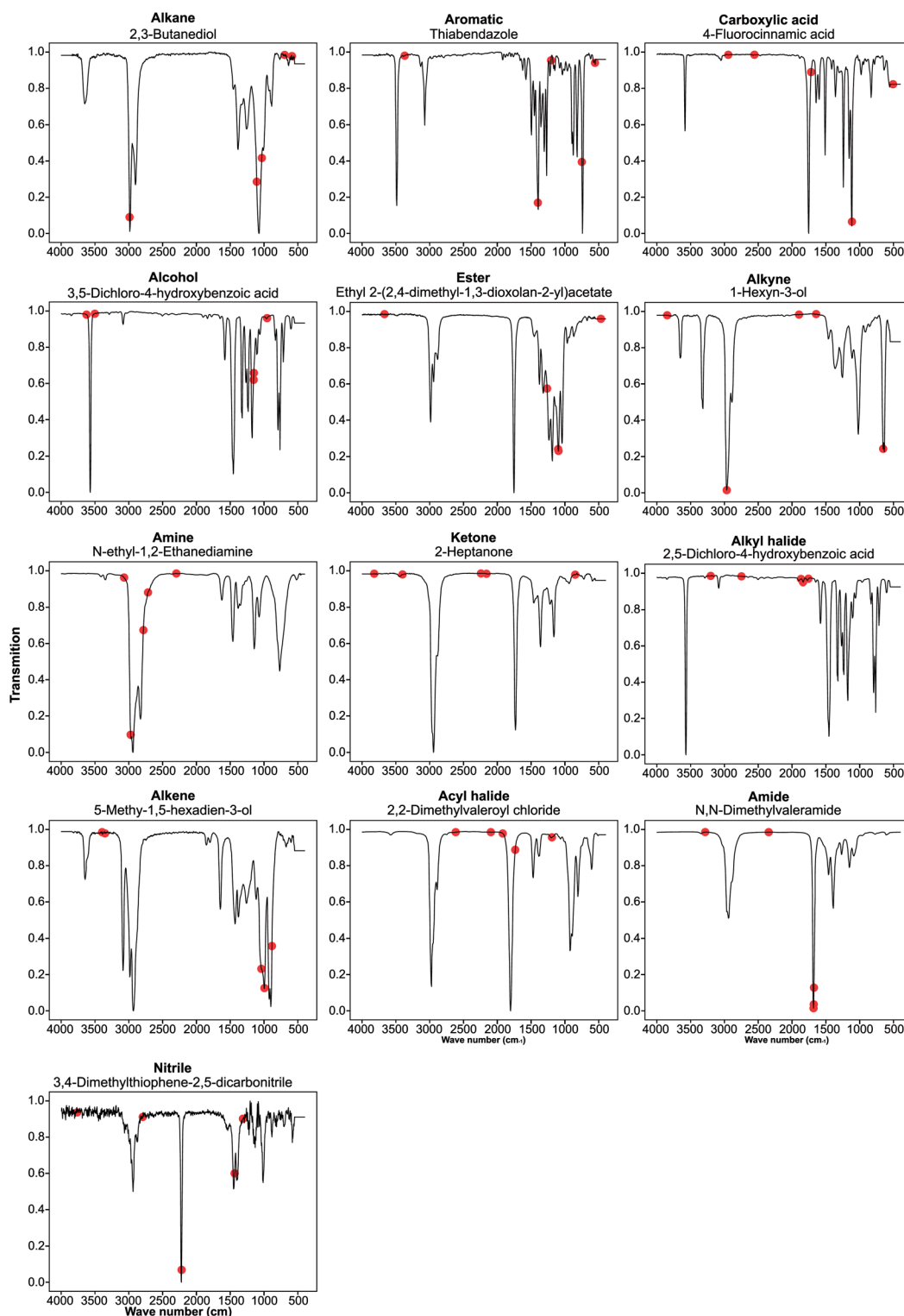
Fig. 4 Backpropagation analysis for all 13 functional groups was performed to identify the regions of the spectra responsible for the result obtained. These plots are listed above in order of decreasing F1 score for the optimised FTIR + MS model.
