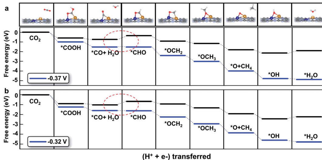
Fig. 5 Free energy diagram of the \text{CO}_2 reduction pathway toward \text{CH}_4 on (a) \text{CuCr}/\text{C}_2\text{N} and (b) \text{CuMn}/\text{C}_2\text{N} at different applied potentials. The potential-limiting steps are marked by red dotted circles.
