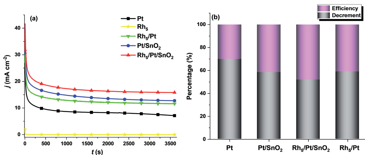
Fig. 6 (a) Durability evaluation by chronoamperometry of electrocatalysts recorded over 1 hour in 1 M \text{C}_2\text{H}_5\text{OH} + 0.5 M \text{H}_2\text{SO}_4 solution. (b) Efficiency and decrement.
