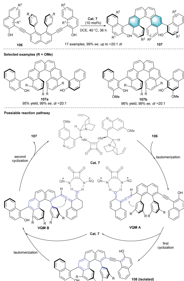
Scheme 30 Bisquinine squaramide-catalyzed intramolecular benzannulation to synthesize chiral helical arenes.
