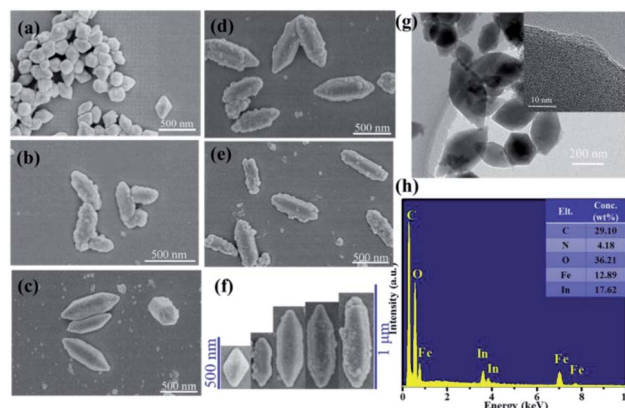
Fig. 2 SEM images of (a) \text{NH}_2\text{-MIL-88B (Fe)} , (b–e) \text{NH}_2\text{-MIL-88B (Fe}_\alpha\text{In}_{1-\alpha}) samples ( \alpha = 0.8, 0.6, 0.4, 0.2 , respectively), (f) the compared SEM images of \text{NH}_2\text{-MIL-88B (Fe}_\alpha\text{In}_{1-\alpha}) , (g) TEM image of \text{NH}_2\text{-MIL-88B (Fe}_{0.6}\text{In}_{0.4}) and (h) EDX image of \text{NH}_2\text{-MIL-88B (Fe}_\alpha\text{In}_{1-\alpha}) .
