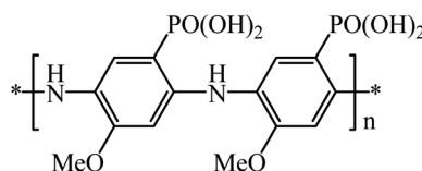
Fig. 9 Poly-2-methoxyaniline-5-phosphoric acid.
