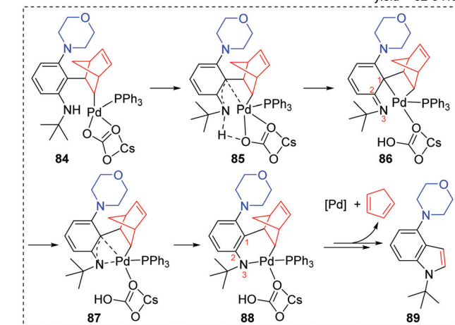
Scheme 18 1,3-Palladium migration that occurred in intramolecular Buchwald coupling.
