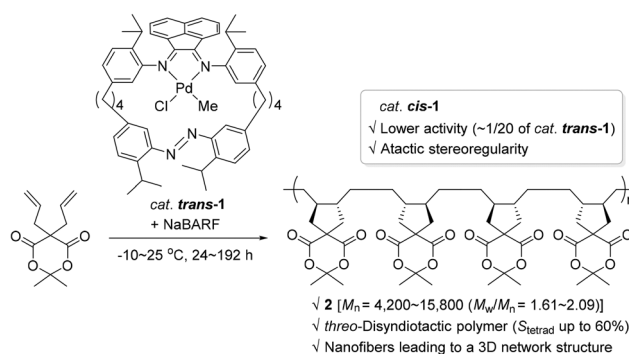
Scheme 2 Cyclopolymerization of isopropylidene diallylmalonate catalyzed by trans - 1 or cis - 1 .
