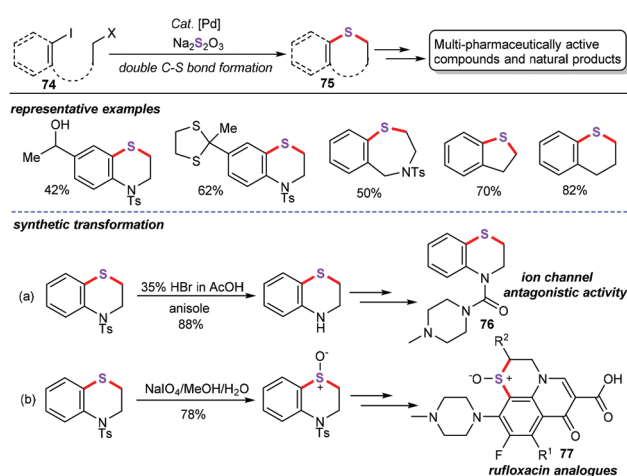
Scheme 29 Palladium-catalyzed double C–S bond formation coupling reaction.
